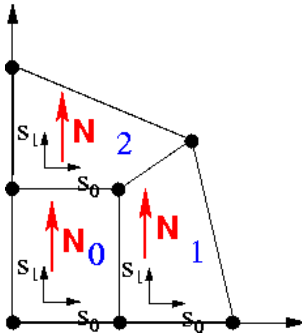
Figure 1.1: Mesh consisting of three RefineableQElements<2>/ QuadTrees. Element/QuadTree numbers are blue, and the QuadTree's 'northern' direction is indicated by the red arrows. The QuadTrees are combined into a QuadTreeForest, which establishes their adjacency (QuadTree 2 is QuadTree 0's northern neighbour etc.) and their relative orientation (QuadTree 1's North coincides with QuadTree 2's West, etc.) Note that the RefineableQElement<2>'s local coordinates s_0 and s_1 are aligned with the QuadTree's W \rightarrow E and S \rightarrow N directions, respectively.
