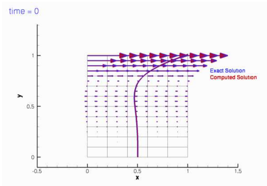
Figure 1.3: Plot of the velocity field computed with 2D Taylor-Hood elements, starting from the exact, time-periodic solution.
