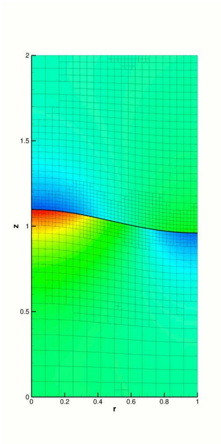
Figure 1.1: Pressure contour plot for the axisymmetric relaxing interface problem.
